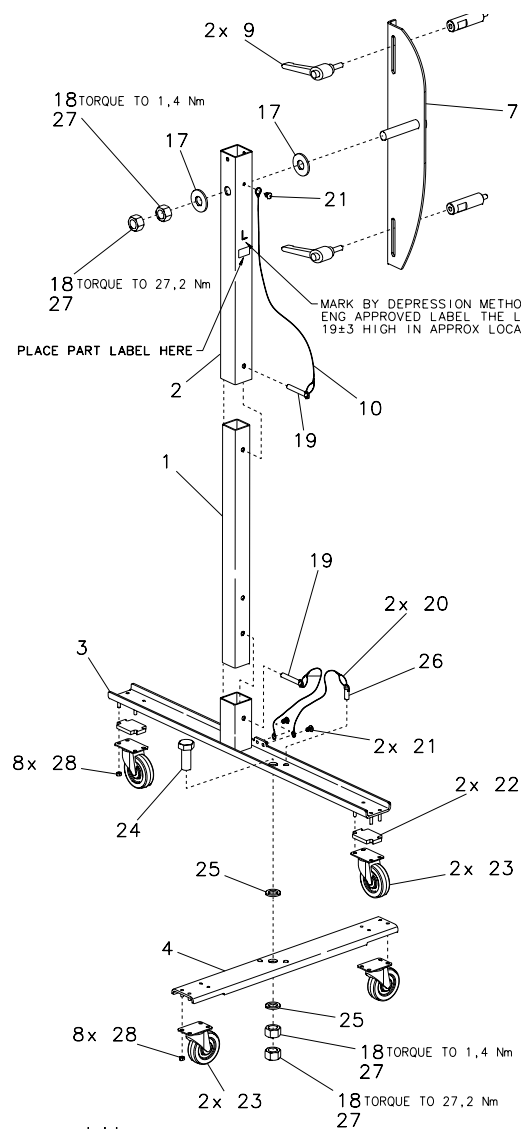
Figure 5-1 Dolly, Pivoting, Small Room (5179183 Sheet 1, Rev 3)
