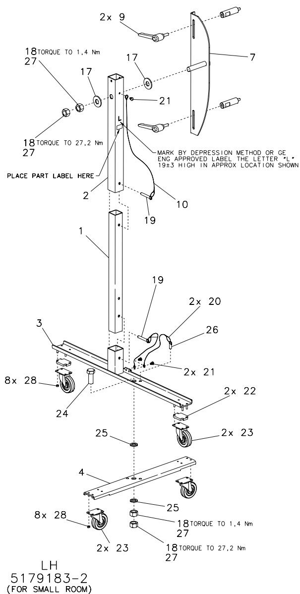
Figure 5-2 Dolly, Pivoting, Small Room (5179183 Sheet 1, Rev 3)
